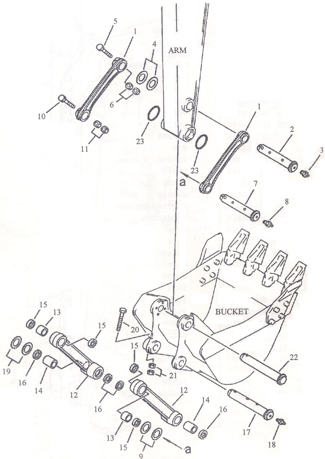
FIG.3 LINK (FOR 40 & 60 FEET LONG FRONT)
