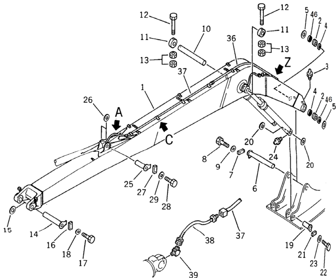
Detail - A
