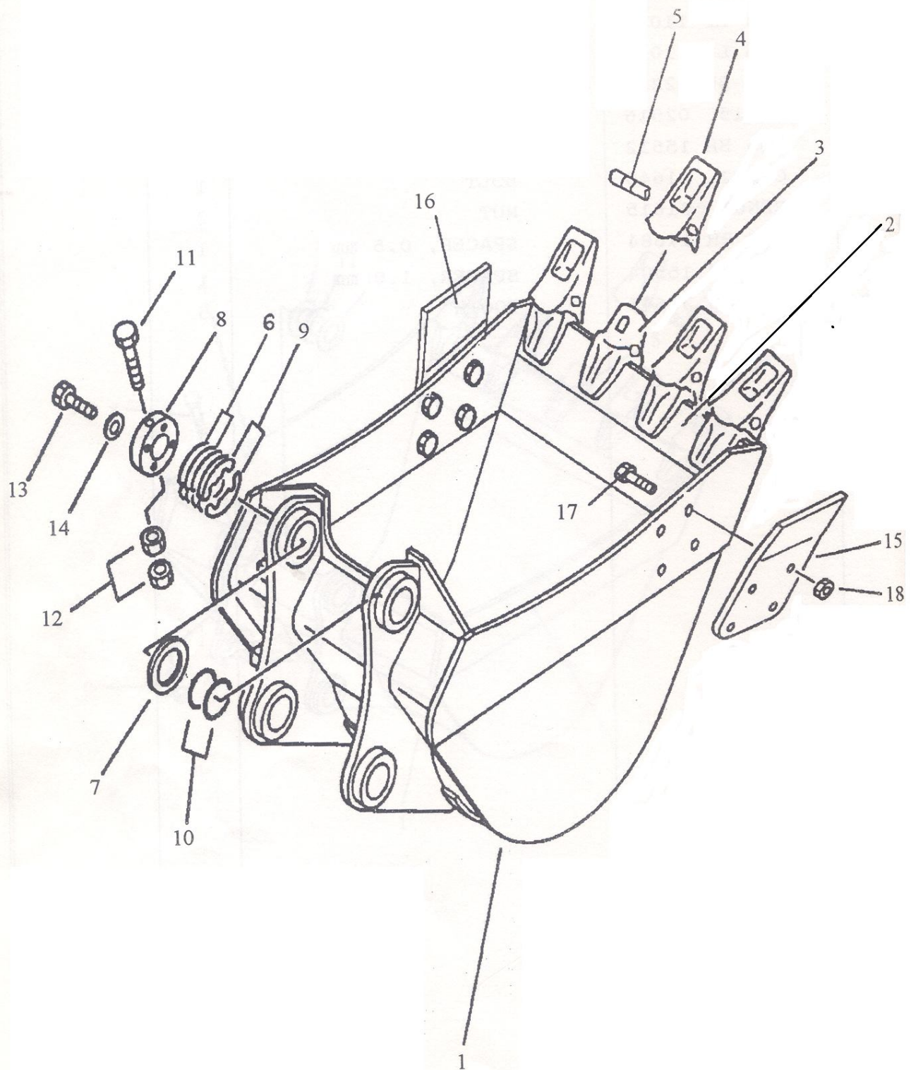
FIG. 9A BUCKET 0.44Cu M SAE (FOR 60 FEET LONG FRONT)
